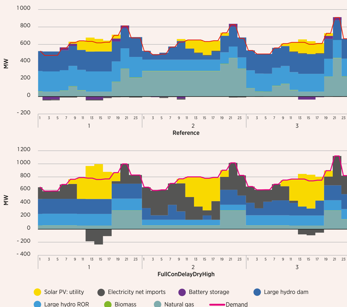
Figure 36 Gabon sub-annual generation mix, 2040 (MW): Reference and FullConDelayDryHigh scenarios
