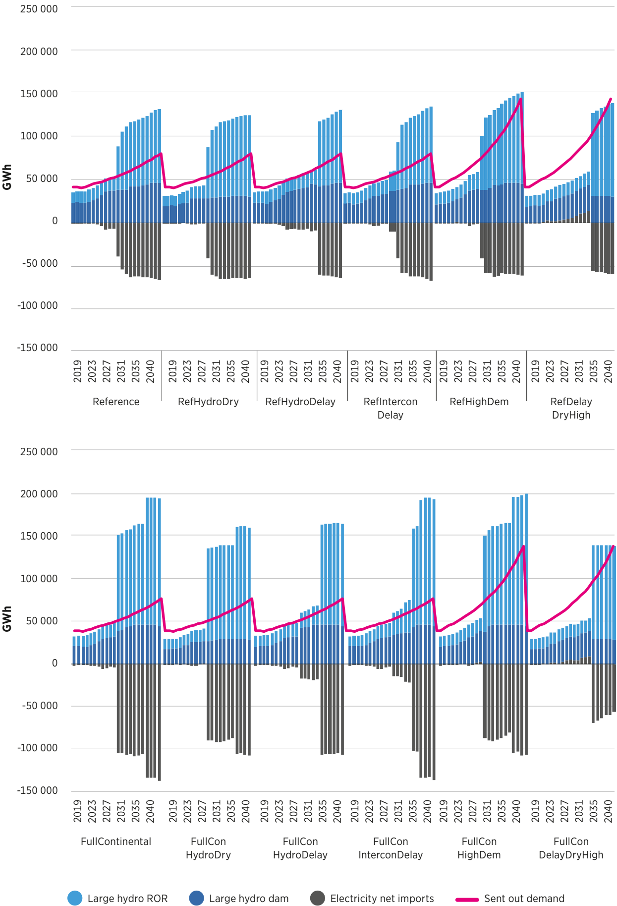
Figure 20 Hydropower production in all scenarios
