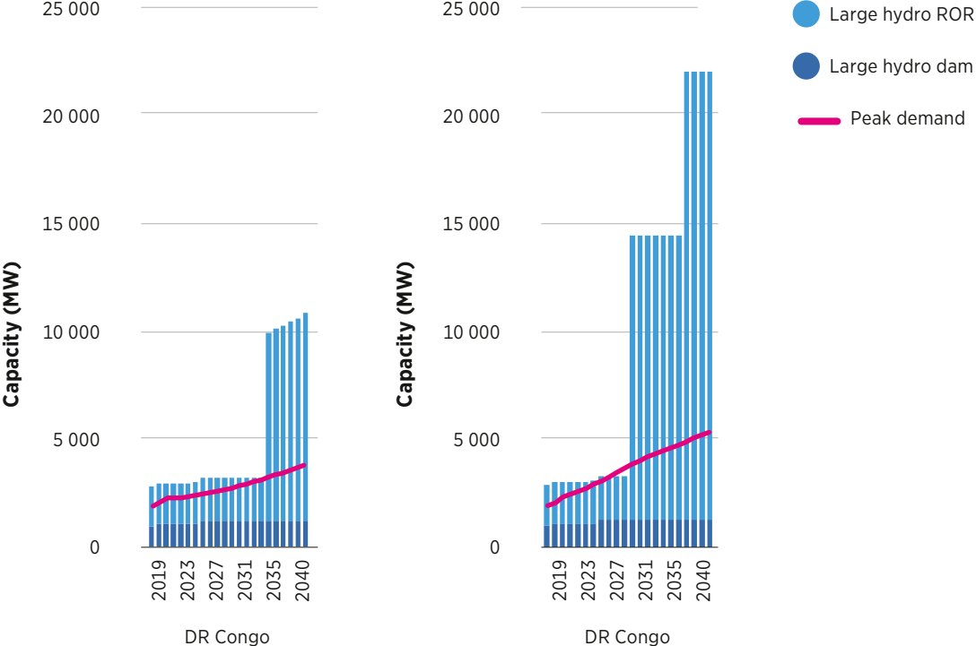
Figure 21 Continued : Democratic Republic of Congo results for hydropower capacity in scenarios with the lowest (RefHydroDelay), left, and the highest (FullConHighDem), right.
