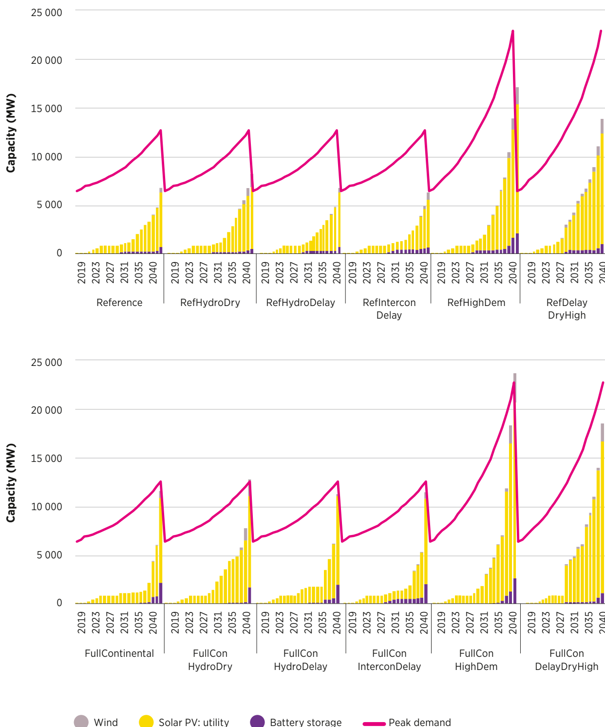
Figure 22 Solar PV, onshore wind and battery capacity across all scenarios
