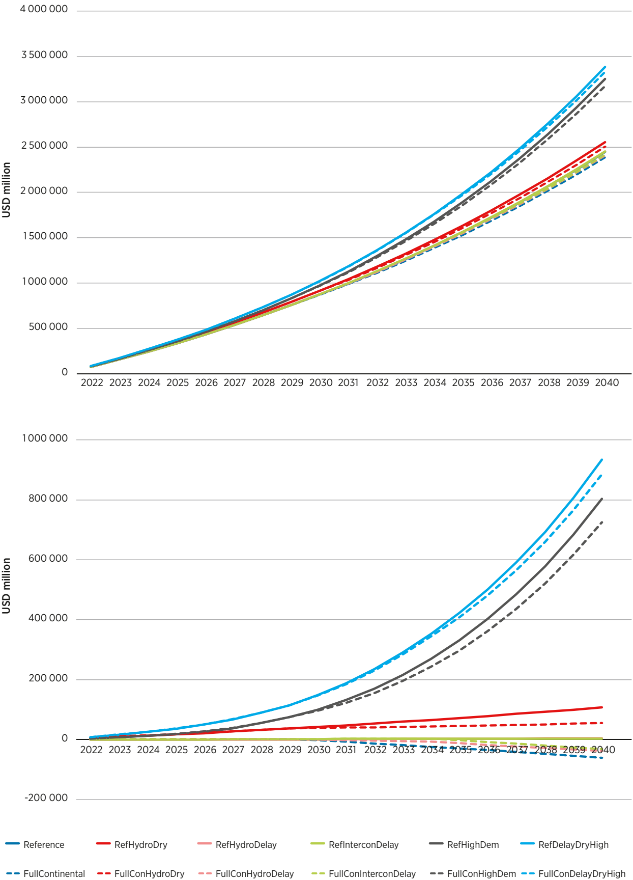
Figure 41 Cumulative total system costs (USD million) by scenario (top) and difference from Reference scenario (bottom), Africa
