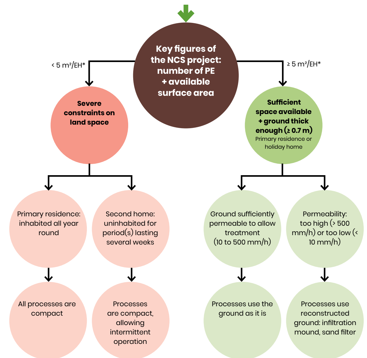
Flowchart for selecting a suitable NCS process for the local context
