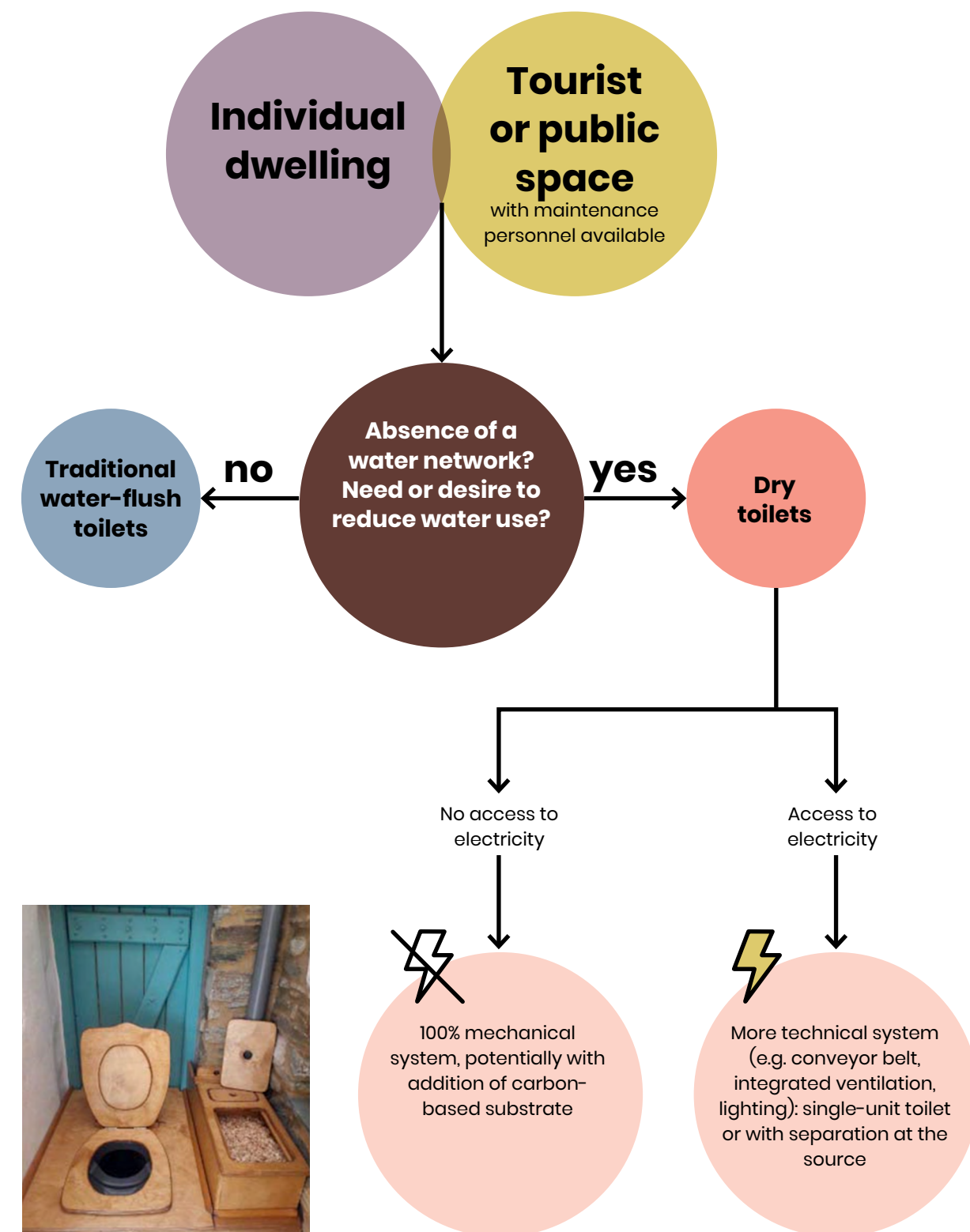
Dry toilets (photo credit: Eric MINO, HYDROUSA or SEMIDE, to be confirmed)
